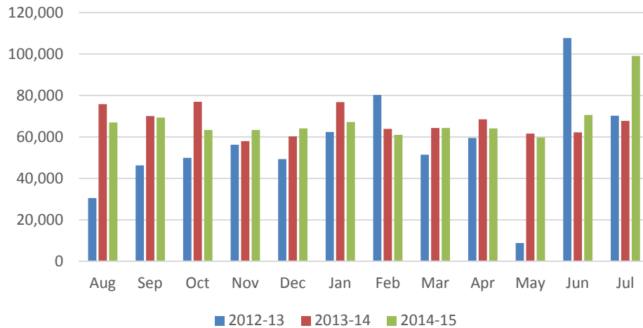
Electricity Usage (kWh)
